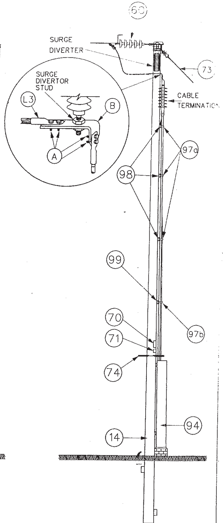
SIDE ELEVATION
